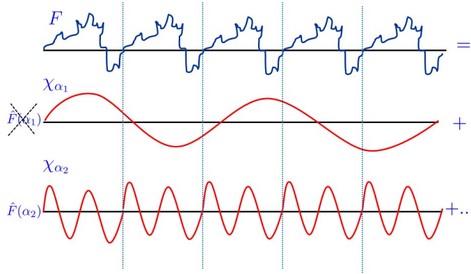
Figure 1: If f is a periodic function then when we represent it in the Fourier transform, we expect the coefficients corresponding to wavelengths that do not evenly divide the period to be very small, as they would tend to “cancel out”.
